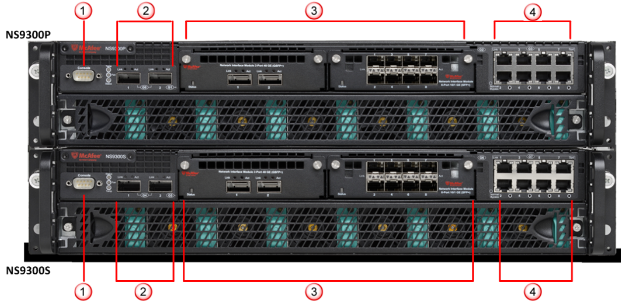
Figure 3 - Front Panels of NS-9300 P (top) and S (bottom)
