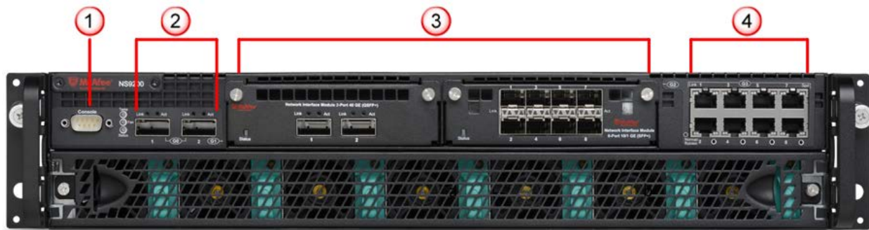
Figure 2 – NS-9100/9200 Front Panel
