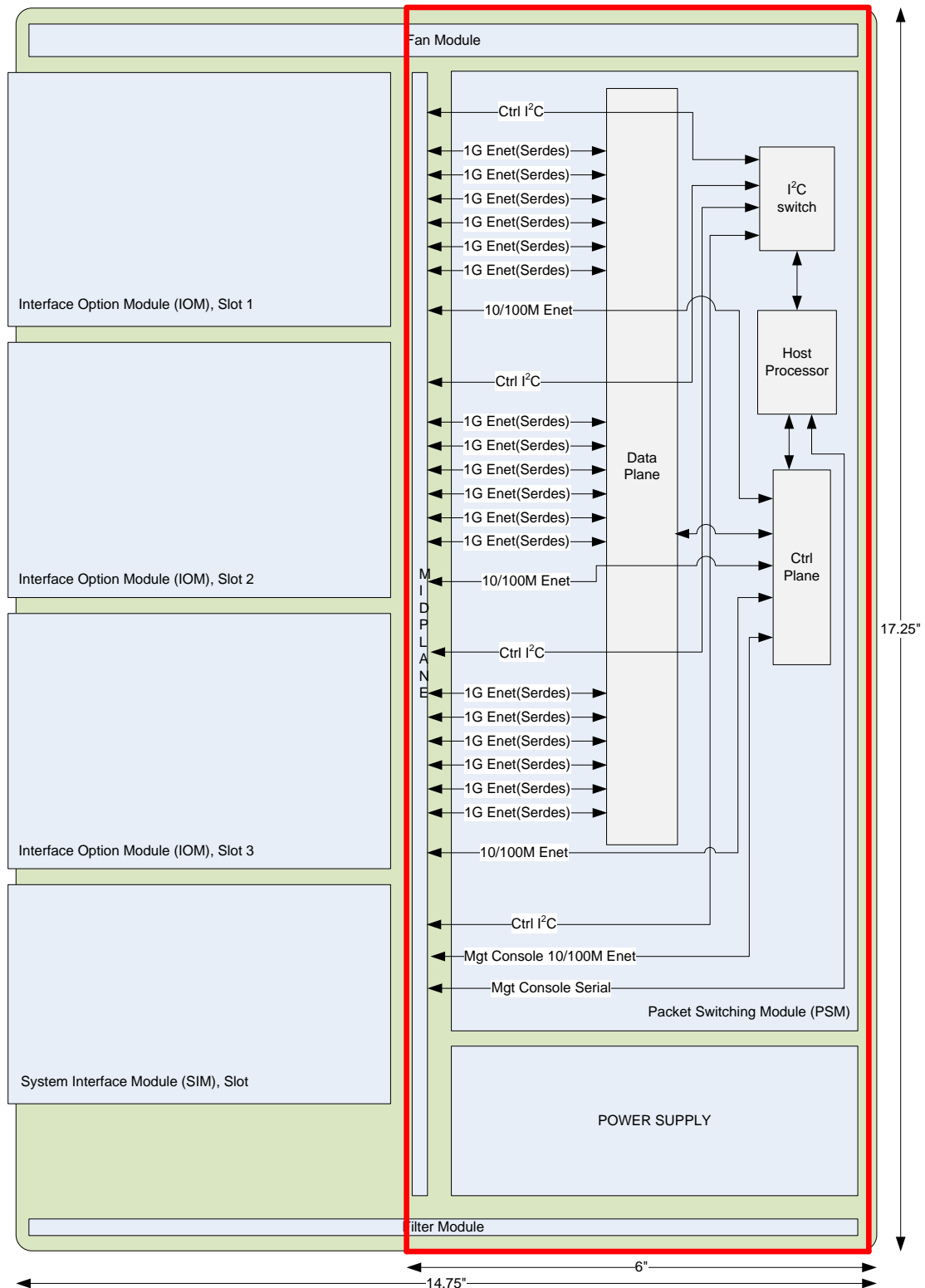
Figure 2 Cryptographic Boundary
