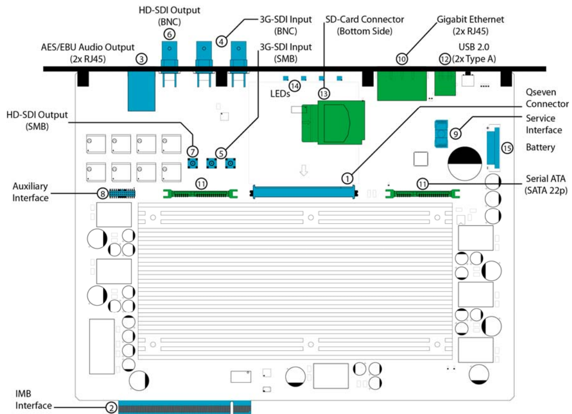
Figure 3 – Physical Connectors
