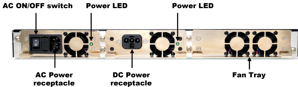
Figure 13 - Rear View: CN6000 Series Encryptor pictured with AC & DC supplies installed
