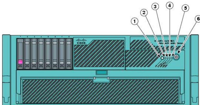
Figure 11 – Cisco ASA 5580 Series Security Appliance Front Panel
