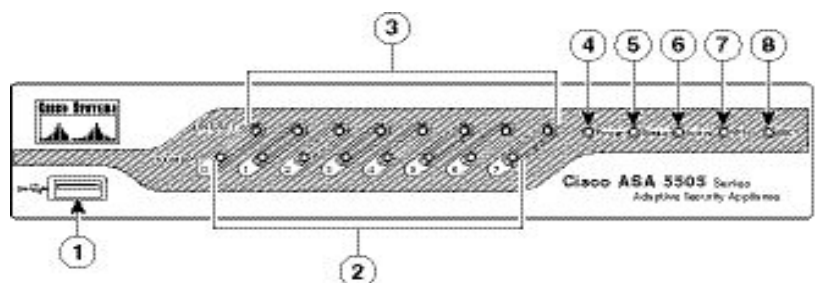
Figure 1 – Cisco ASA 5505 Series Security Appliance Front Panel
