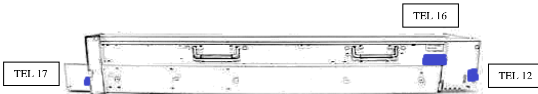
Figure 35 Cisco ASA 5580 Security Appliance Tamper Evident Label Placement (Side Face)
