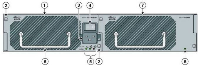
Figure 17 – Cisco ASA 5585-X Series Security Appliance Rear Panel
