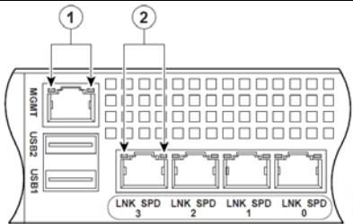
Figure 10 – Cisco ASA 5510, 5520, 5540 and 5550 Series Security Appliance Rear Panel Link and Speed Indicator
