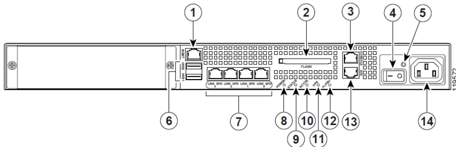
Figure 4 – Cisco ASA 5510, 5520, 5540 Series Security Appliance Rear Panel
