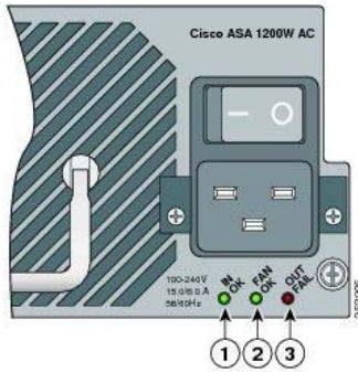
Figure 18 – Cisco ASA 5585-X Series Security Appliance Rear Panel Indicators
