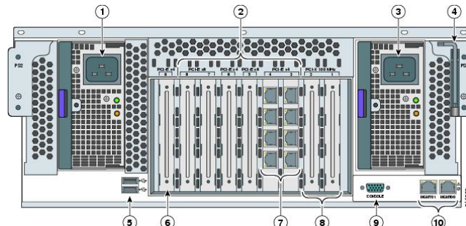
Figure 13 – Cisco ASA 5580 Series Security Appliance Rear Panel
