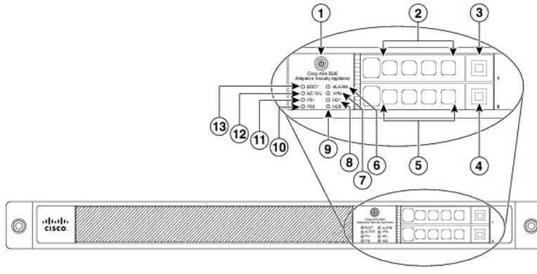
Figure 7 – Cisco ASA 5545 and 5555 Series Security Appliance Front Panel
