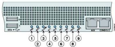
Figure 16 – Cisco ASA 5585-X Series Security Appliance Rear Panel Indicators
