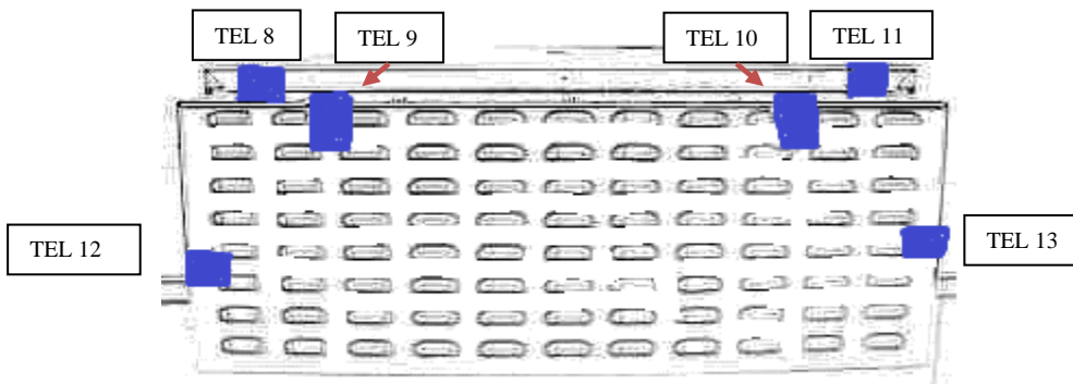
Figure 33 Cisco ASA 5580 Security Appliance Tamper Evident Label Placement (Back Face)
