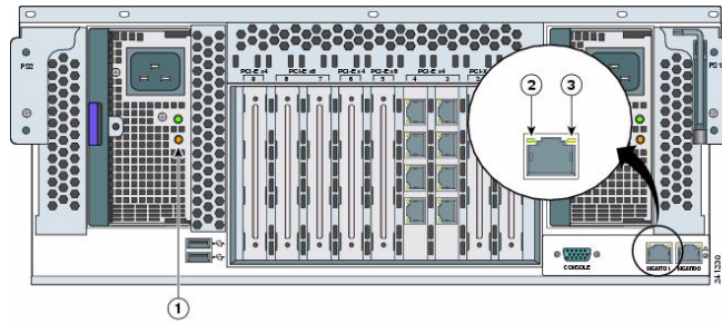
Figure 12 – Cisco ASA 5580 Series Security Appliance Rear Panel Indicators
