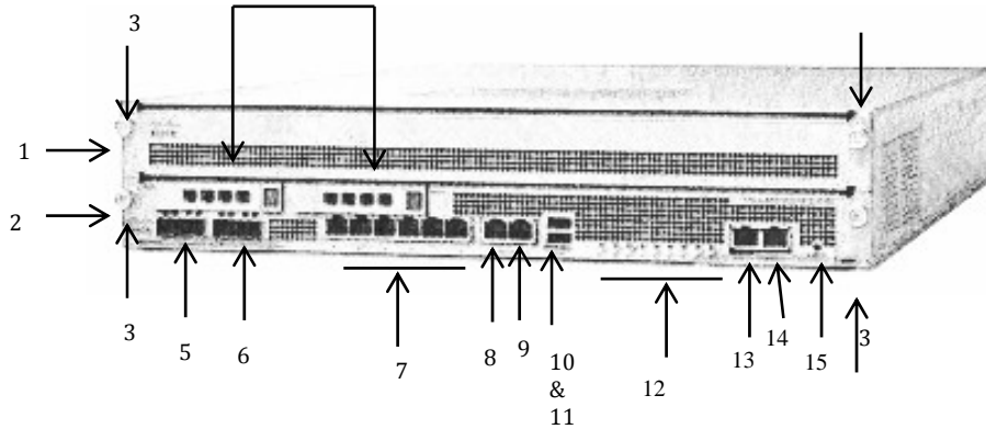
Figure 15 – Cisco ASA 5585-X SSP-40 and SSP-60 Series Security Appliance Front Panel
