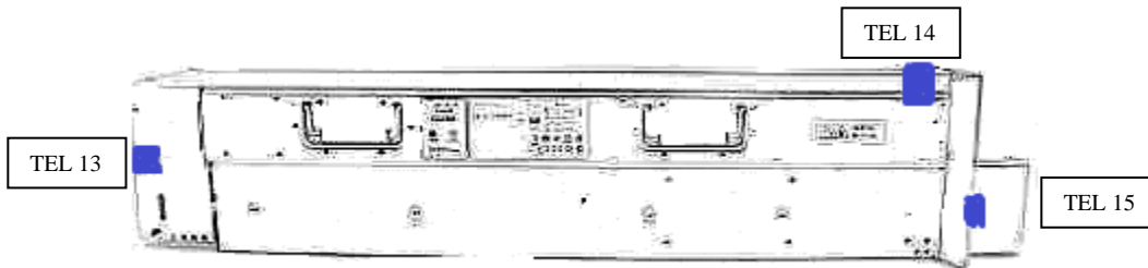
Figure 34 Cisco ASA 5580 Security Appliance Tamper Evident Label Placement (Side Face)
