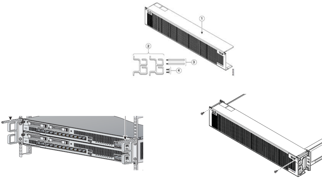
Figure 22 – ASA 5585-X Front Opacity Shield Placement
