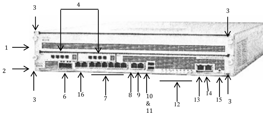
Figure 14 – Cisco ASA 5585-X SSP-10 and SSP-20 Series Security Appliance Front Panel
