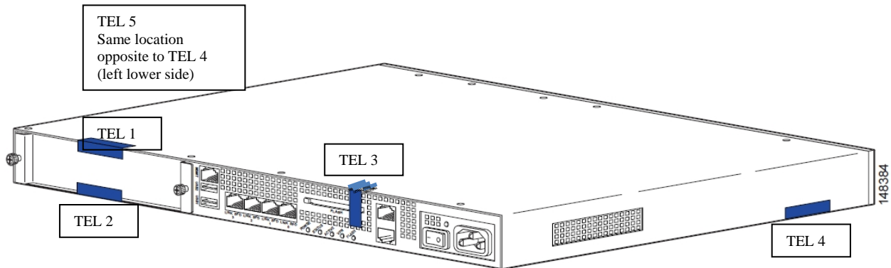
Figure 25 Cisco ASA 5510, 5520, and 5540 Security Appliance Tamper Evident Label Placement
