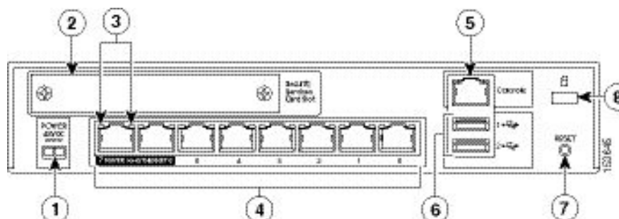
Figure 2 – Cisco ASA 5505 Series Security Appliance Rear Panel
