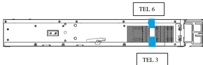
Figure 40 Cisco ASA 5585 Security Appliance with Tamper Evident Label Placement (Left Face)
