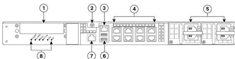
Figure 8 – Cisco ASA 5545 and 5555 Series Security Appliance Rear Panel
