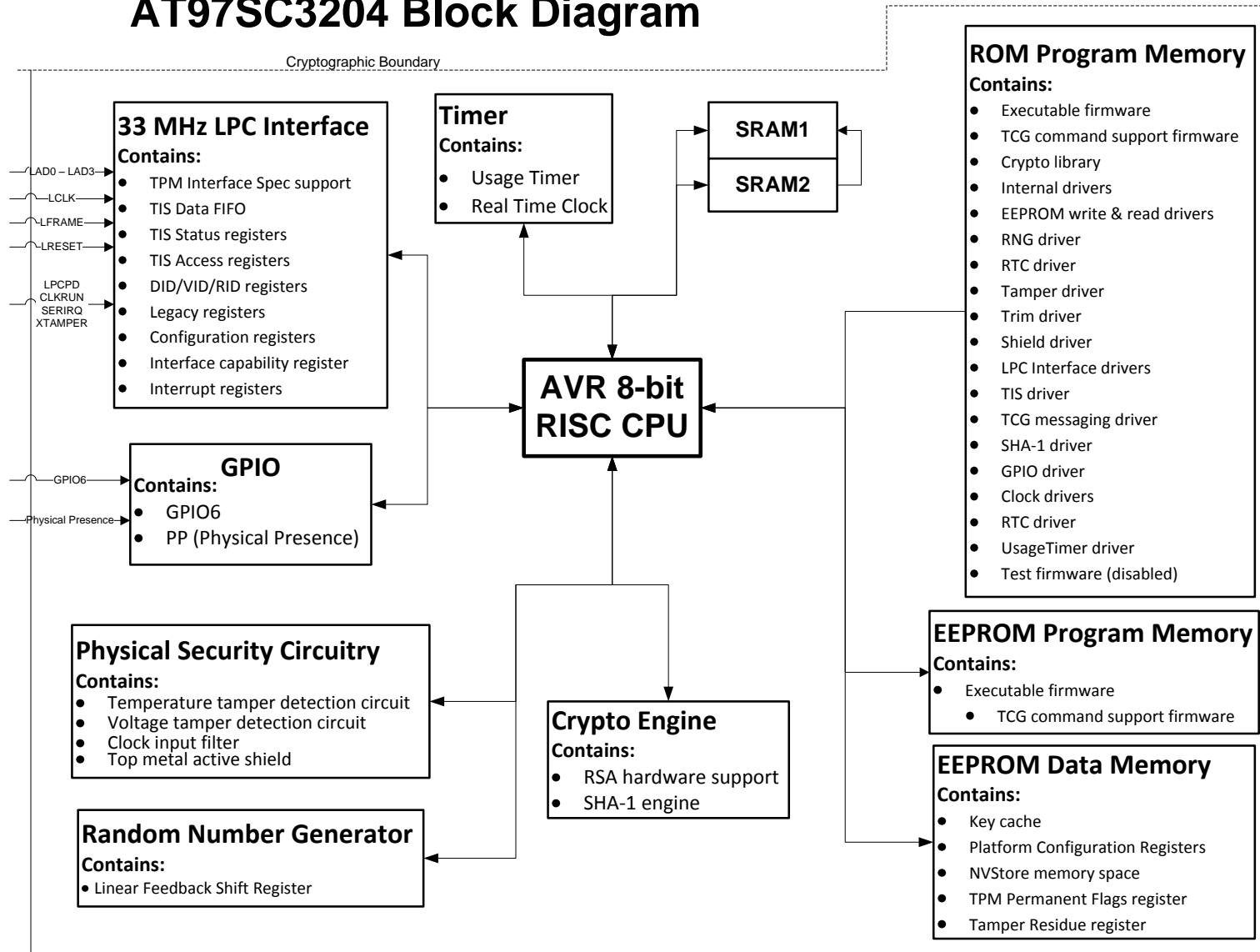
Figure 1 AT97SC3204-X4 Block Diagram
