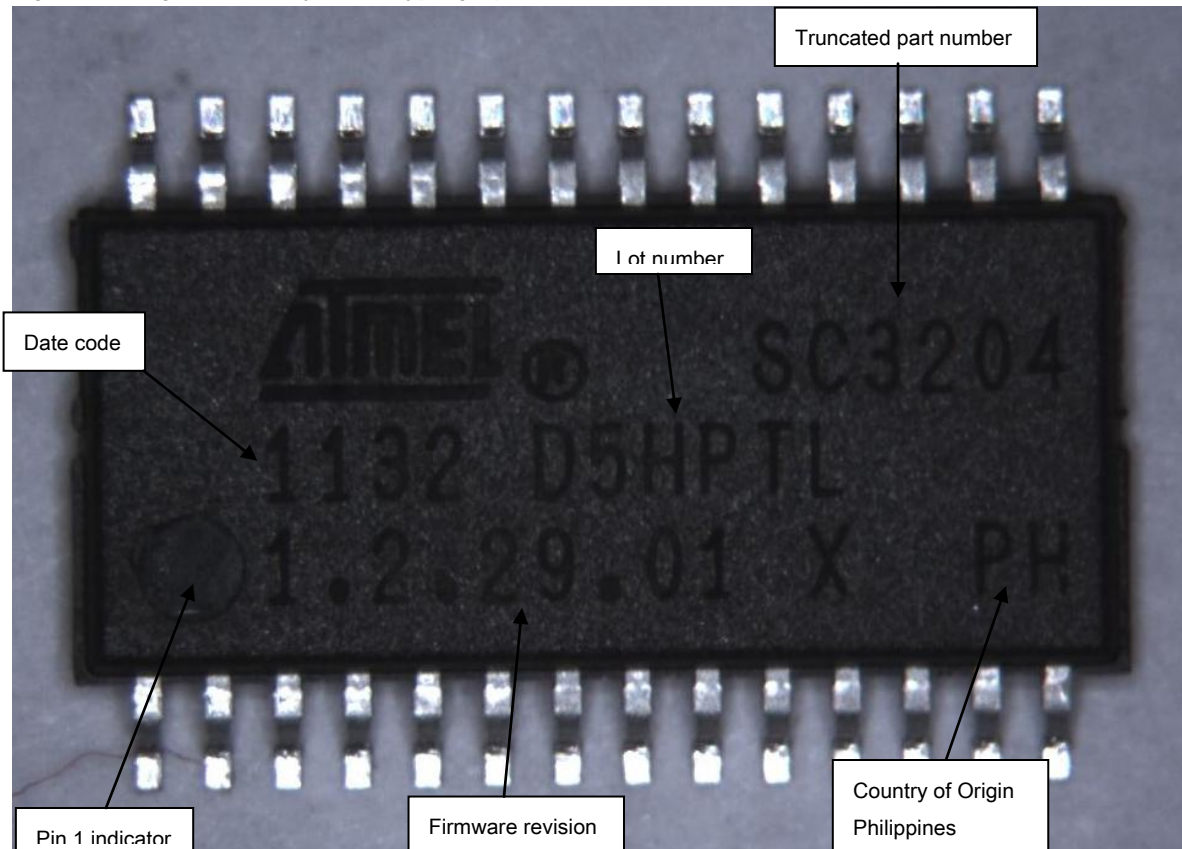
Figure 2 Image of the Physical Cryptographic Module
