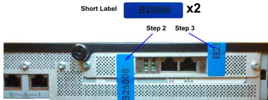
Figure 15 Tamper Evident Label Placement for the NIC Interface Cutout
