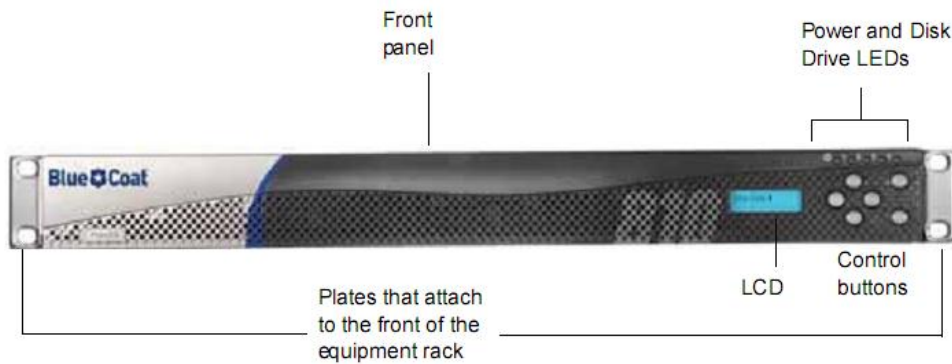
Figure 5 Front View of the ProxySG 810
