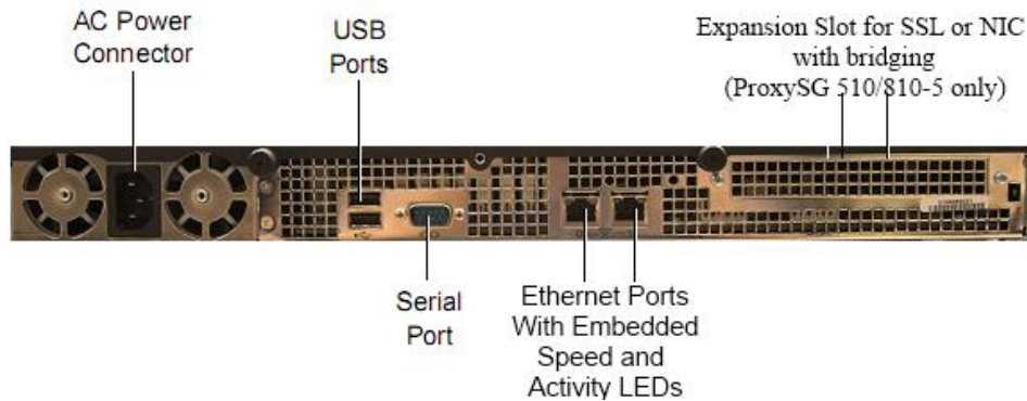
Figure 6 Connection Ports at the Rear of the ProxySG 510/810-5
