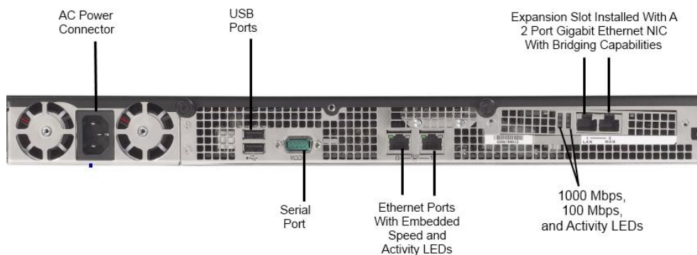
Figure 7 Connection Ports at the Rear of the ProxySG 510/810-10, 20, 25
