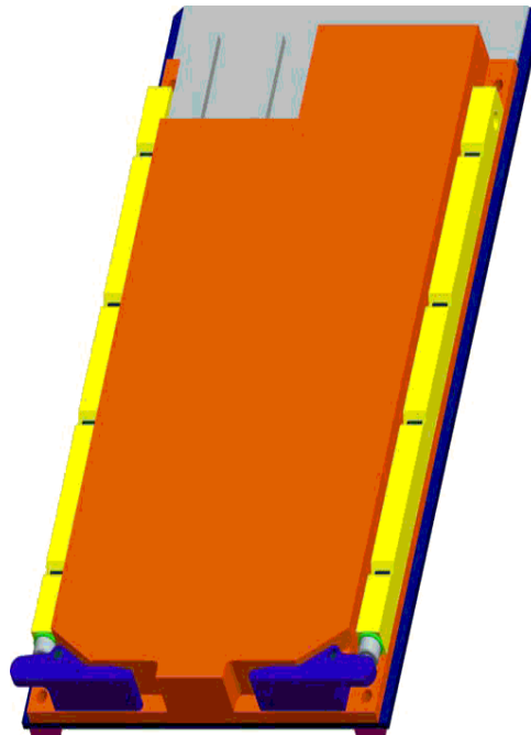
Figure 4: Conduction Cooled cover
