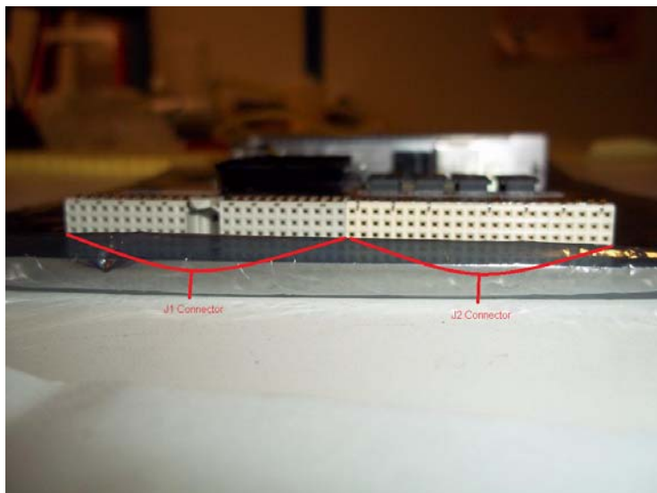
Figure 5: Connector pins
