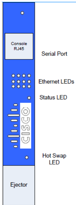
Figure 3: Faceplate
