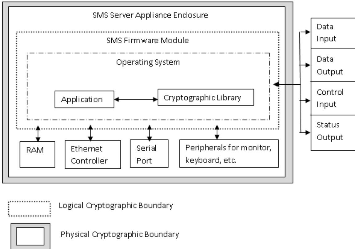
Figure 2: Cryptographic Boundary
