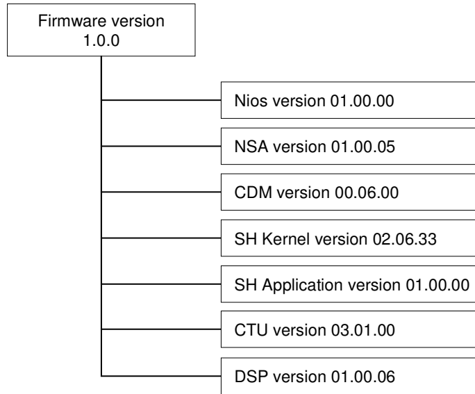
Figure 2 – Gemini firmware configuration.
