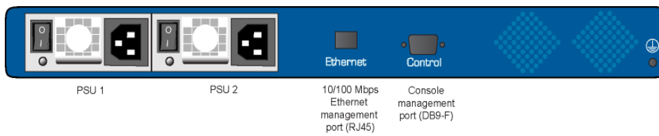
Figure 4-3 1600X427 Front
