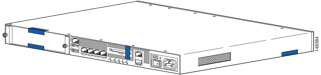
Figure 4 Cisco ASA 5500 Series Security Appliance Tamper Evident Label Placement
