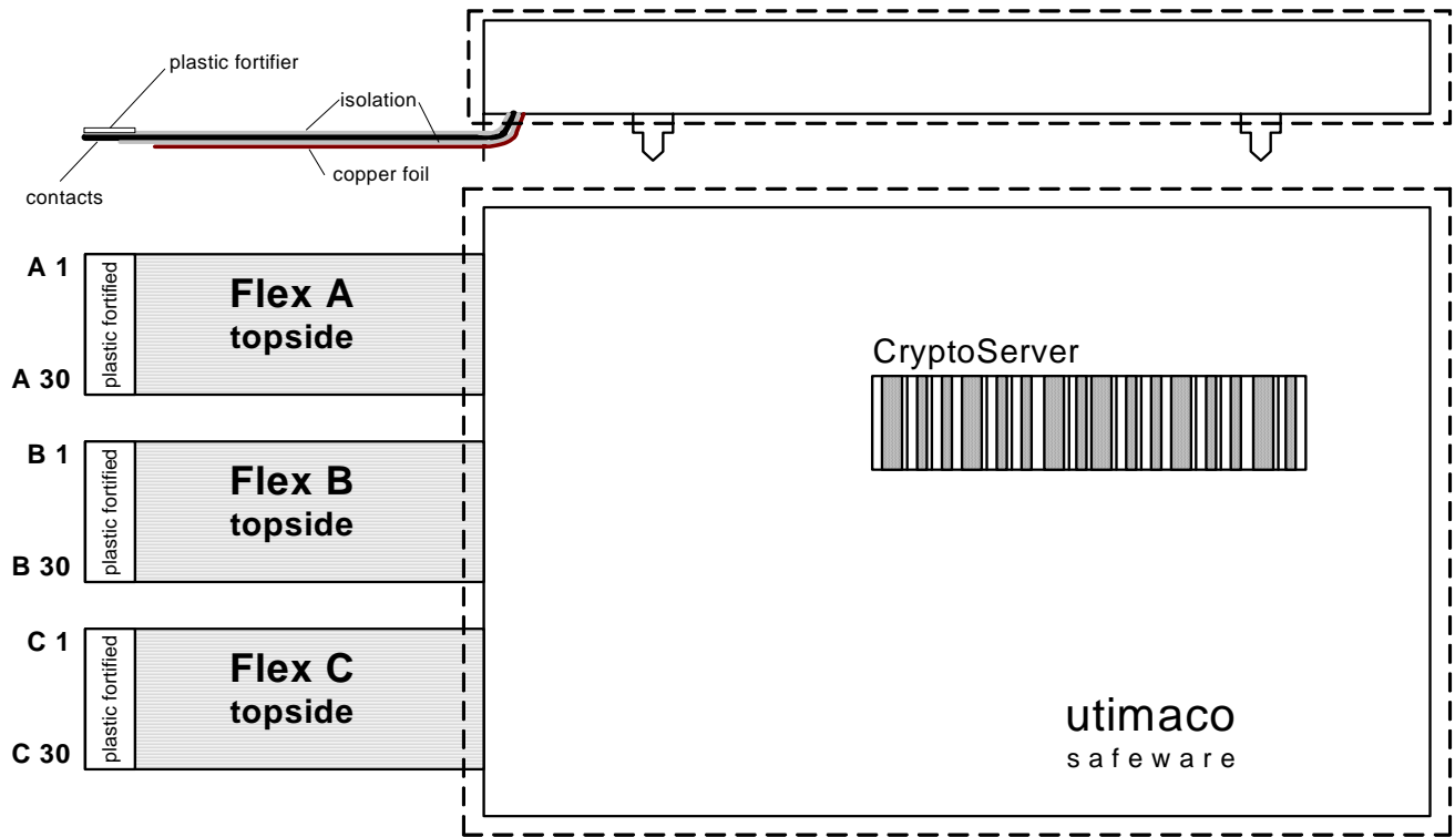
Figure 1 – CryptoServer CS (the dashed line indicates the cryptographic boundary)
