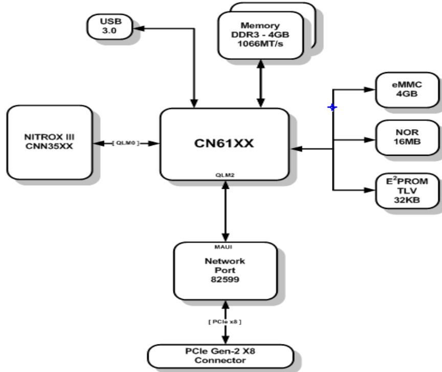
Figure 2 – Block Diagram
