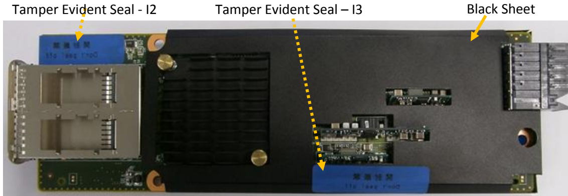
Figure 9 – Top Side of the Module without Metal Frame (HW Version B/D4)
