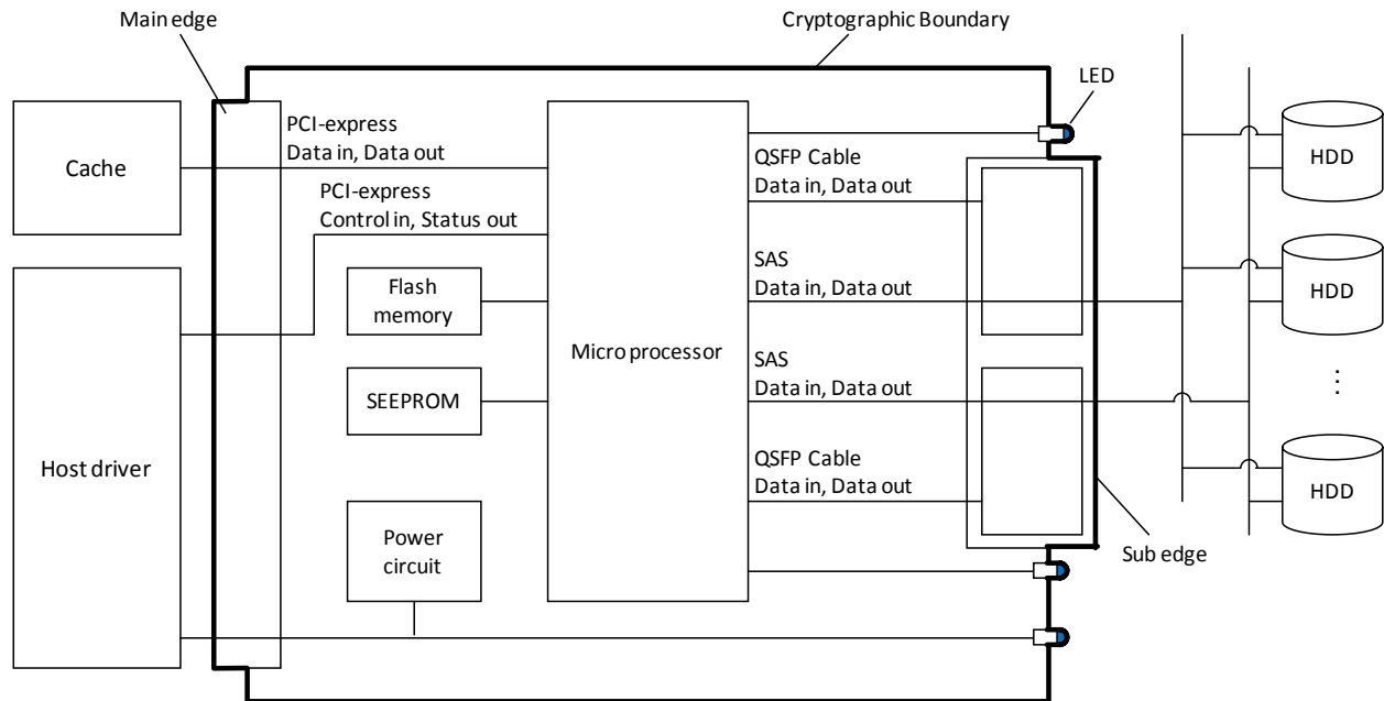
Figure 13 – Module Block Diagram
