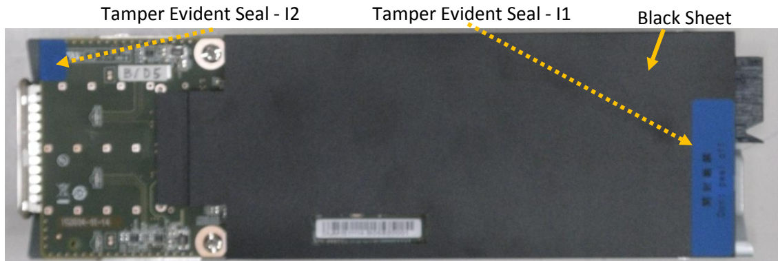
Figure 12 – Bottom Side of the Module without Metal Frame (HW Version B/D5)
