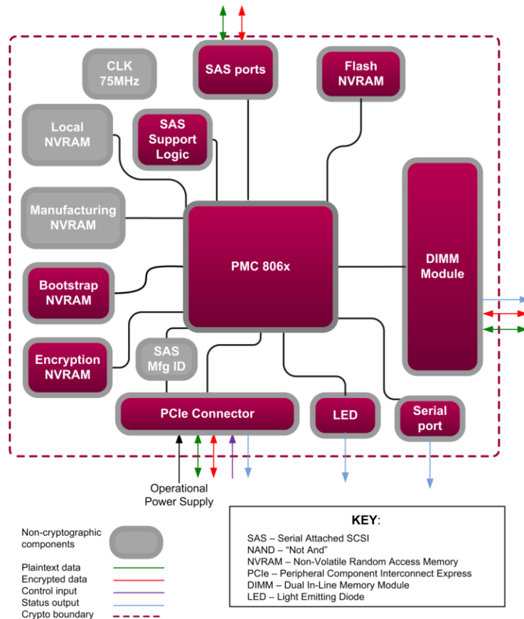
Figure I – HP Smart Array Block Diagram
