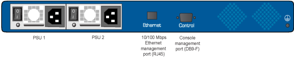
Figure 4-3 1600X437, Rev. 02 Front
