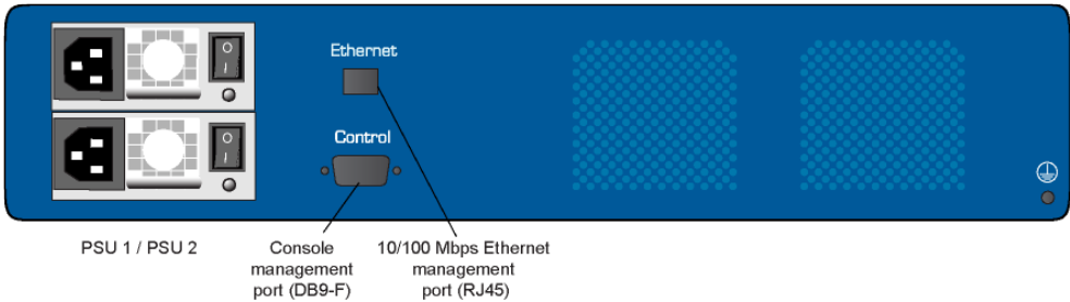
Figure 4-4 1600X437, Rev. 02 Rear
