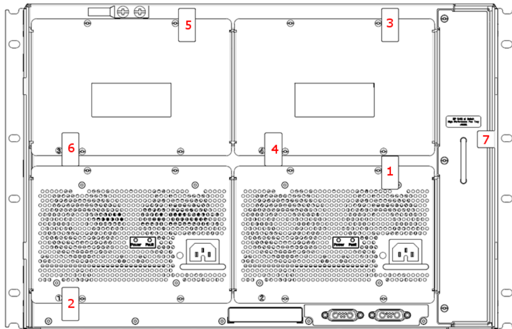
Figure 24 – 5412 zl Rear Tamper-Evidence Label Placement
