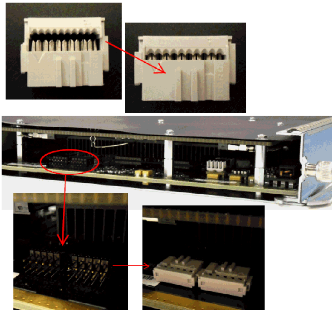
Figure 7 Ten-pin Mating Connectors: Assemble and install on left side of the module
