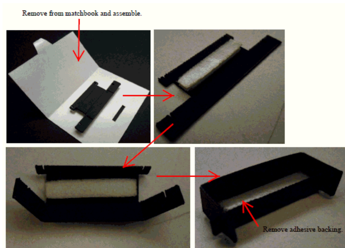
Figure 9 Assembling the Folding Cap
