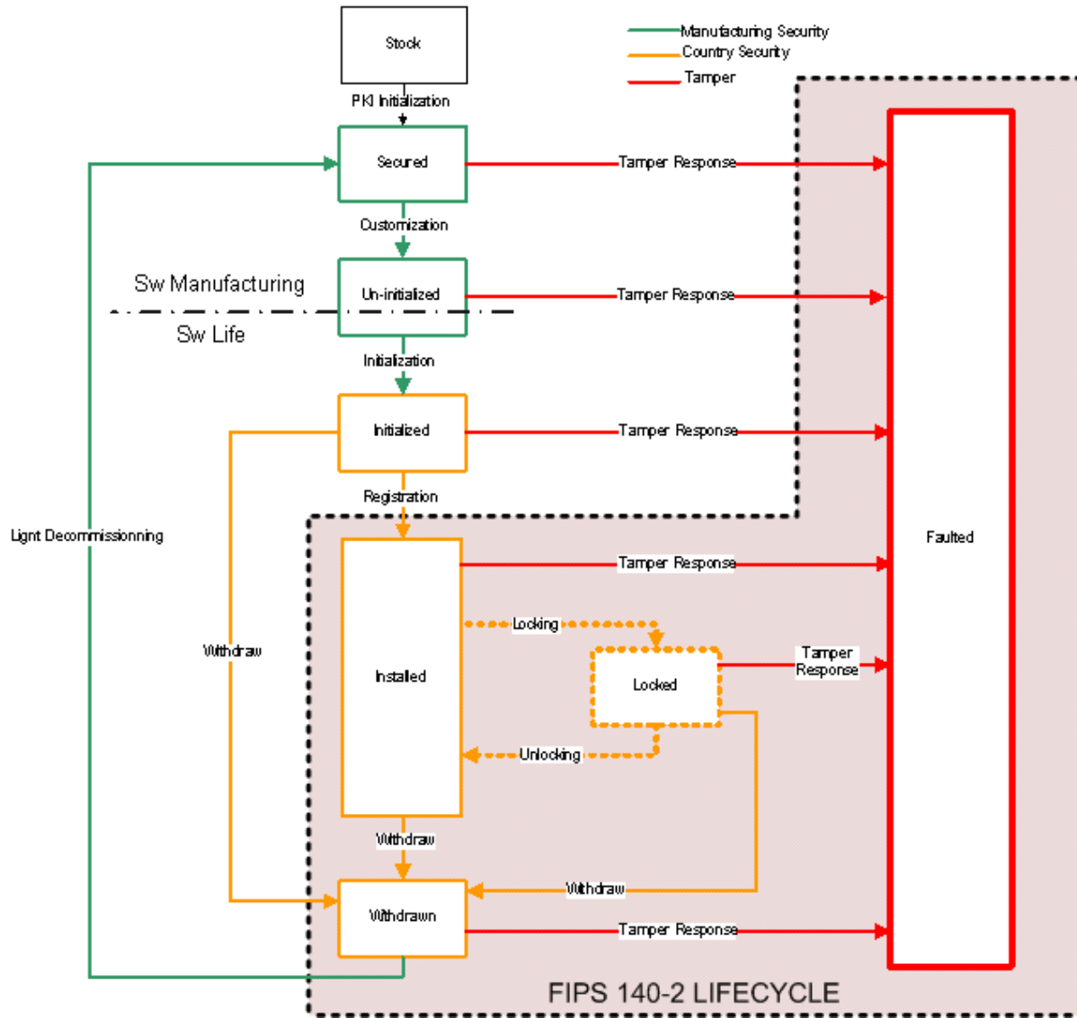
Figure 2 PSD Lifecycle
