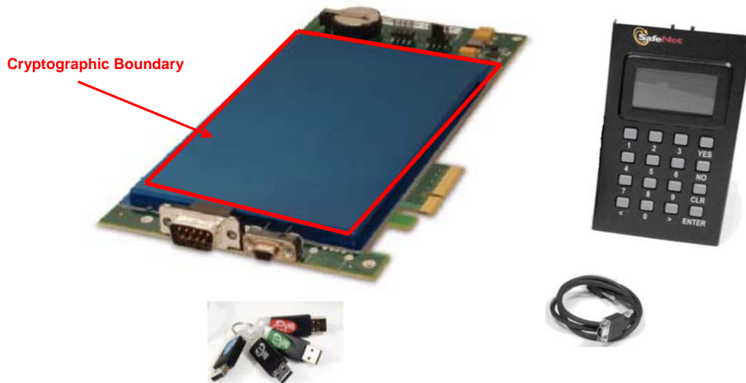
Figure 2-1 Luna PCI-e Cryptographic Module with iKeys and Luna PED
