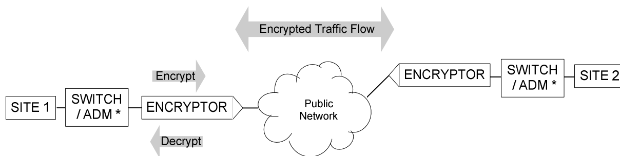
Figure 1. Encryptor Operation.
