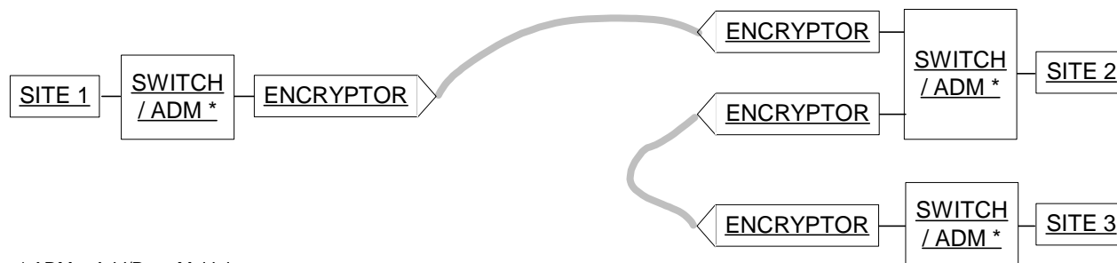
Figure 2. Encryptor Usage Example in Line Encryption Mode.
