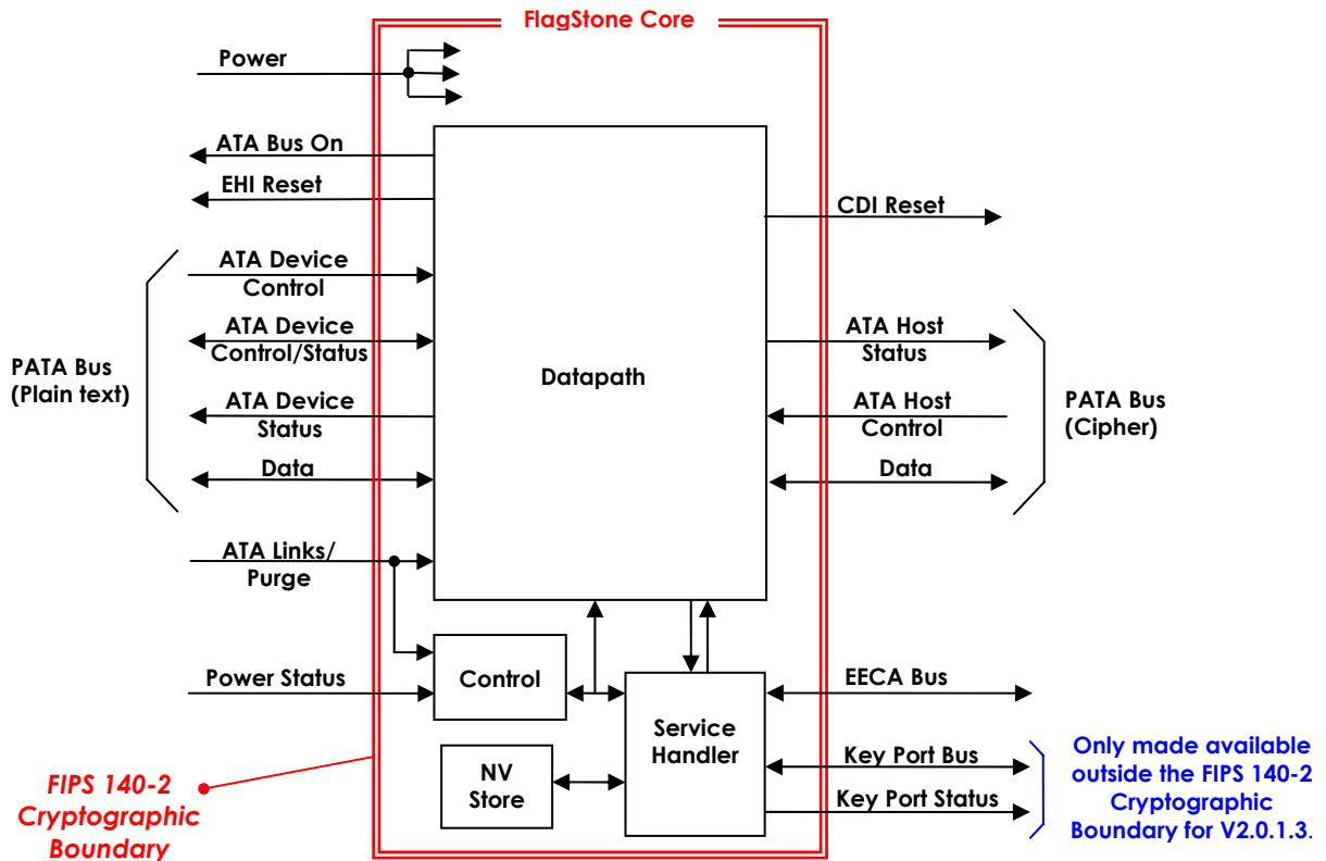
Figure 7 - FlagStone Core Simplified Block Diagram
