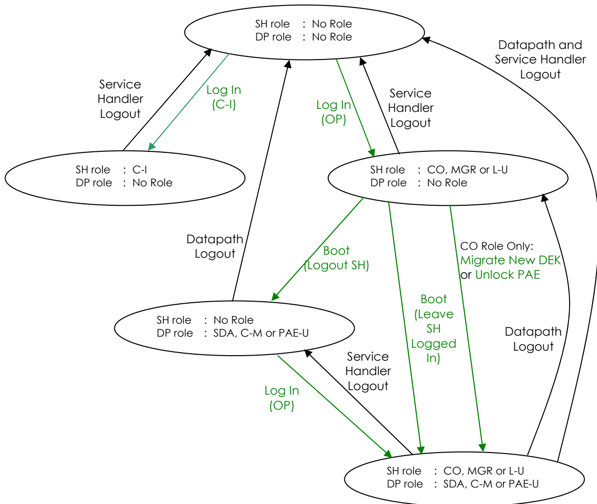
Figure 8 - Session Model (FIPS 140-2 Mode of Operation)
