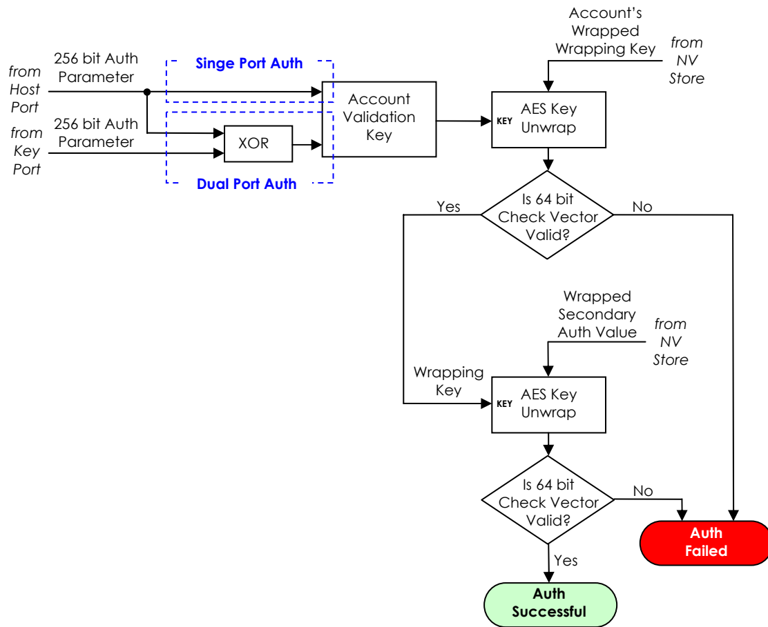
Figure 9 - Authentication Mechanism
