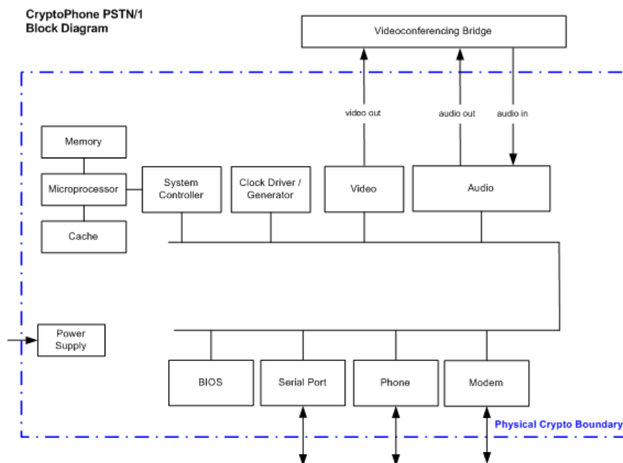
Figure 4 – CryptoPhone PSTN/1 Block Diagram
