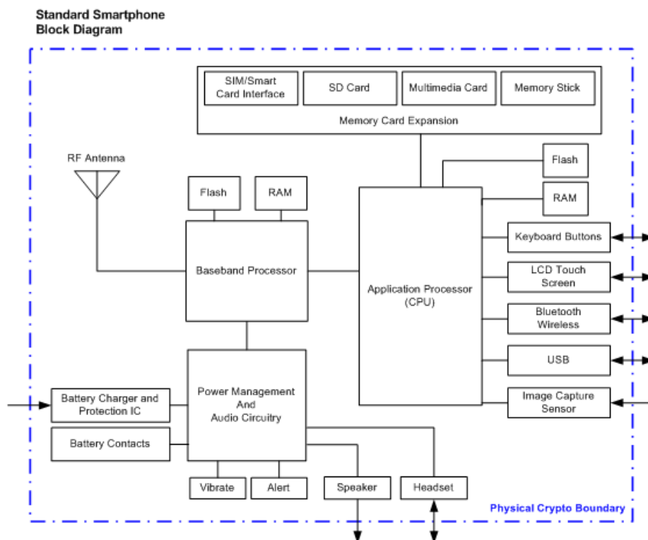
Figure 2 – Standard Smartphone Block Diagram
