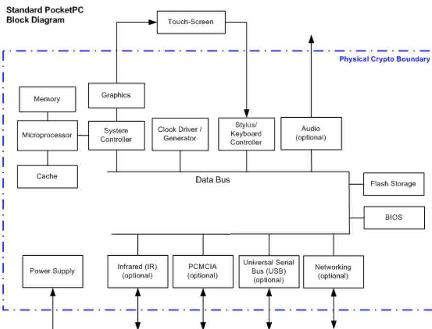
Figure 3 – Standard PocketPC Block Diagram
