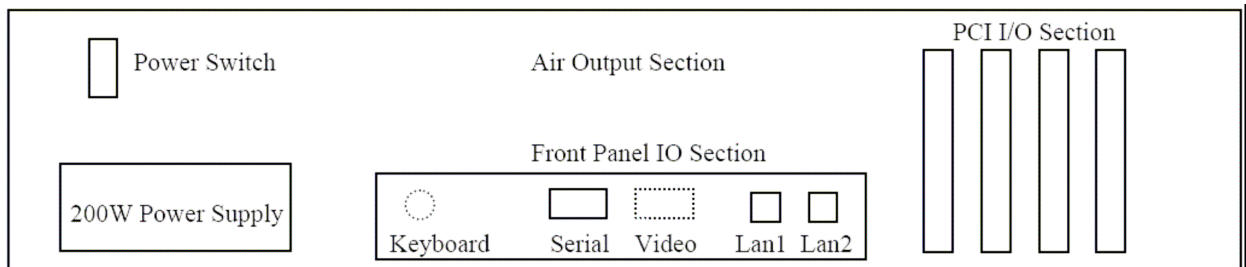
Figure 5 – VPN Router 2750 Rear Panel Physical Ports
