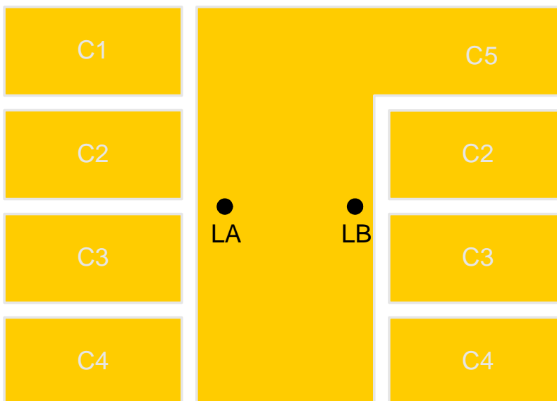
Figure 3 - Contact plate example - Contact-less antenna contacts
